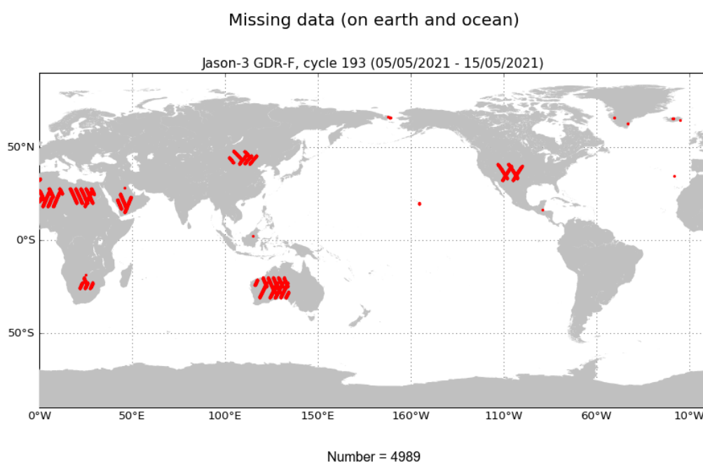
FIGURE 1 – Missing measurements for cycle 193.
