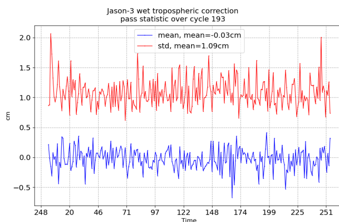
FIGURE 11 – Pass monitoring of wet troposphere differences between radiometer and ECMWF model for Jason-3 cycle 193
