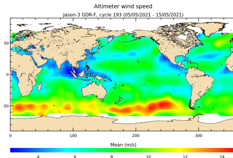
FIGURE 9 – Altimeter wind speed for cycle 193.
