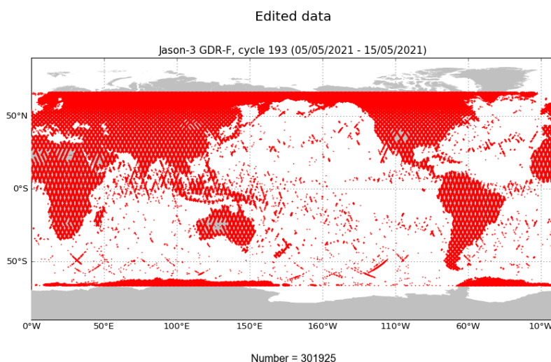
FIGURE 2 – Edited measurements for cycle 193.
