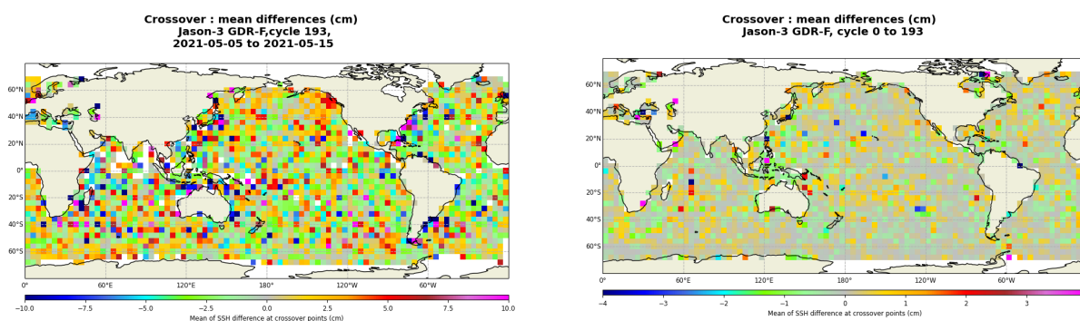
FIGURE 13 – Mean SSH at crossovers for cycle 193 (left) and over the whole Jason-3 period (right).
