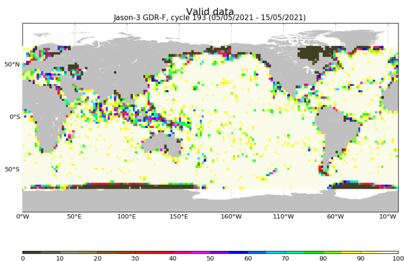
FIGURE 3 – Percentage of valid measurements for cycle 193.
