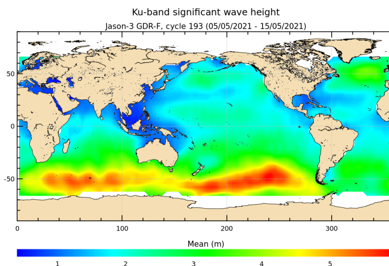
FIGURE 5 – Significant wave height for cycle 193.
