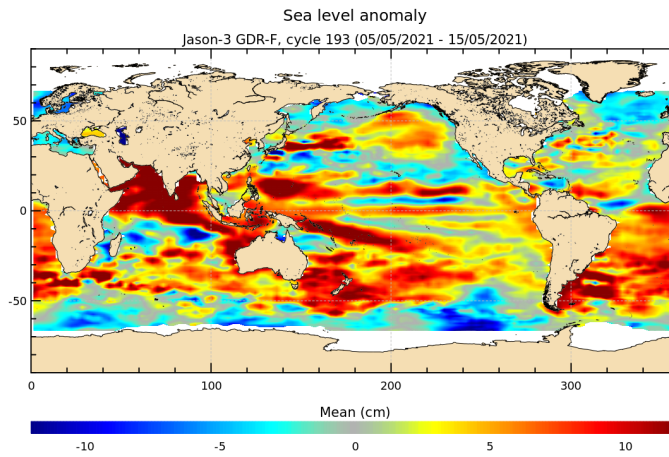
FIGURE 18 – Sea level anomaly relative to MSS for cycle 193.
