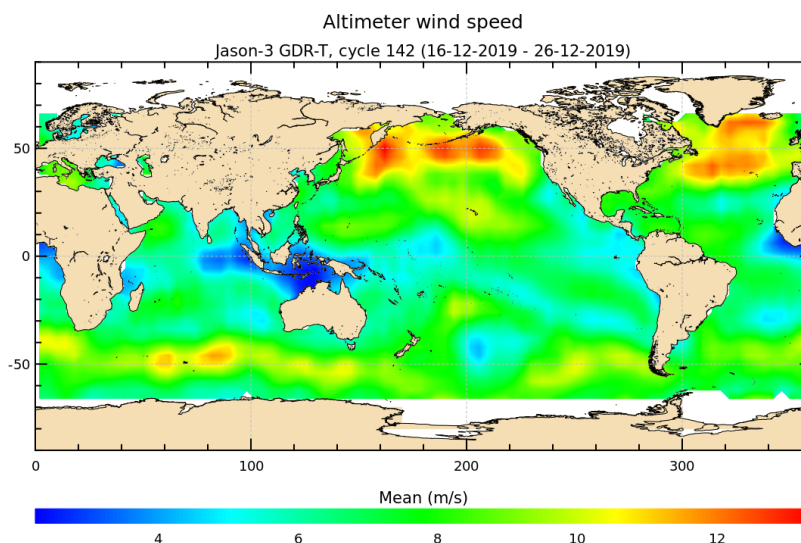
FIGURE 9 – Altimeter wind speed for cycle 142.
